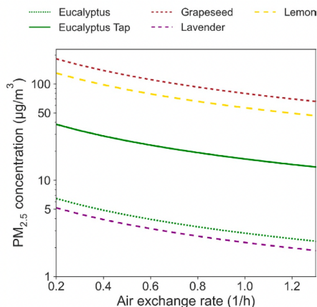
Figure 8. Estimated indoor PM 2.5 concentration due to the use of an essential oil diffuser under varied air change rates. Dashed lines indicate expected concentrations when the diffuser is filled with deionized water, and solid lines indicate expected values when the diffuser is filled with tap water.
